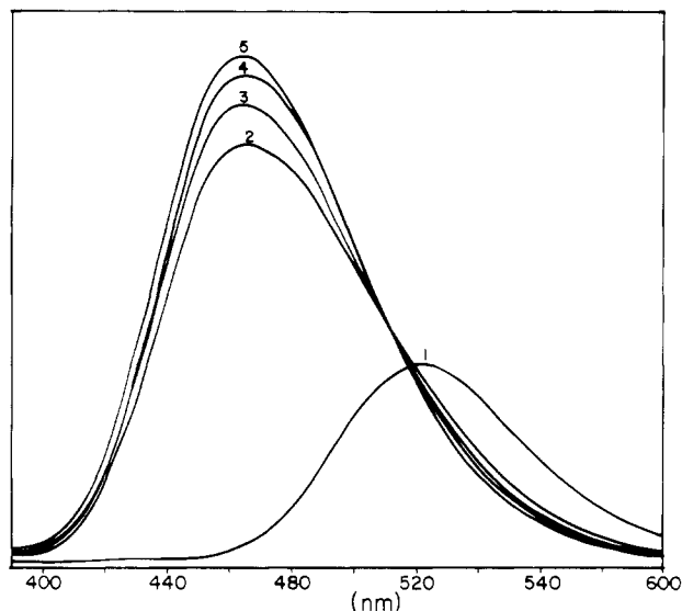
FIGURE 4: Fluorescence spectrum of PRODAN in water at 3 \mu M concentration. 2, 3, 4, and 5 are for the same PRODAN concentration and respectively 38, 75, 150, and 300 \mu M bovine serum albumin (excitation at 350 nm).
